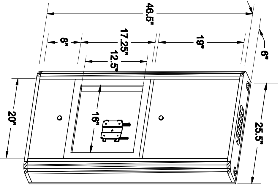
ISOMETRIC VIEW
